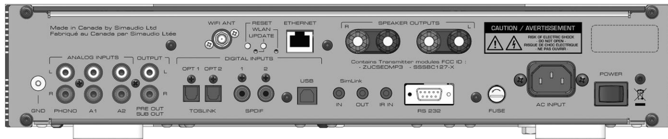
Figure 2: ACE Rear panel
